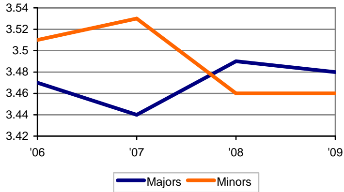
Average GPA for Majors and Minors
