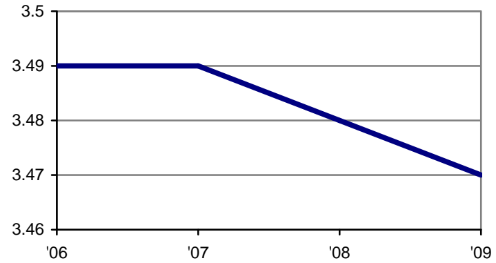
Average Undergraduate GPA
